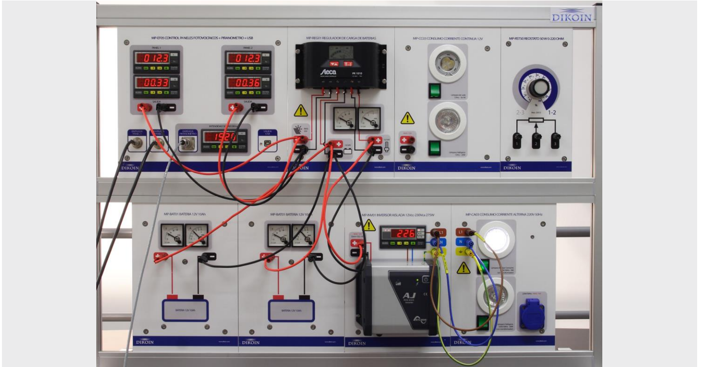
The wiring system through 4mm safety terminals allows a fast and secure connection for the students
